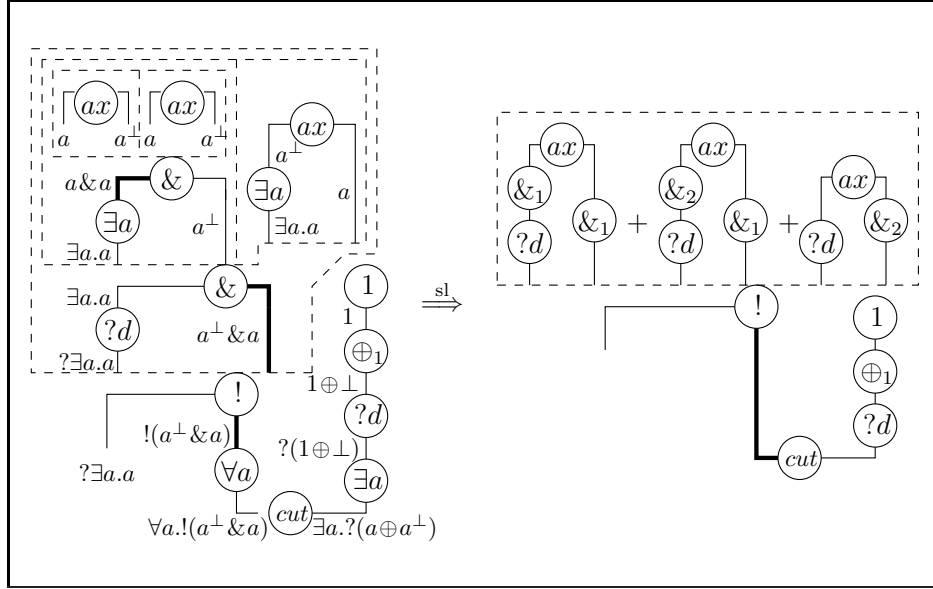
Figure 21: An example of slicing a net
