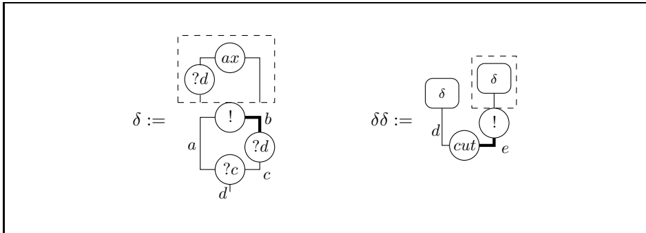
Figure 9: The slice \delta\delta which is not WN
