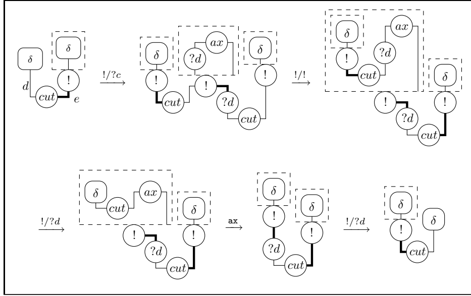
Figure 10: A proof that \delta\delta \xrightarrow{cut+} \delta\delta
