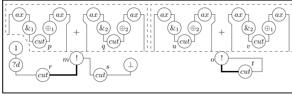
Figure 3: An example of sps
