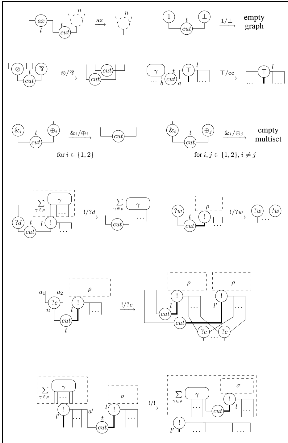
Figure 5: The reduction steps for cut-elimination
