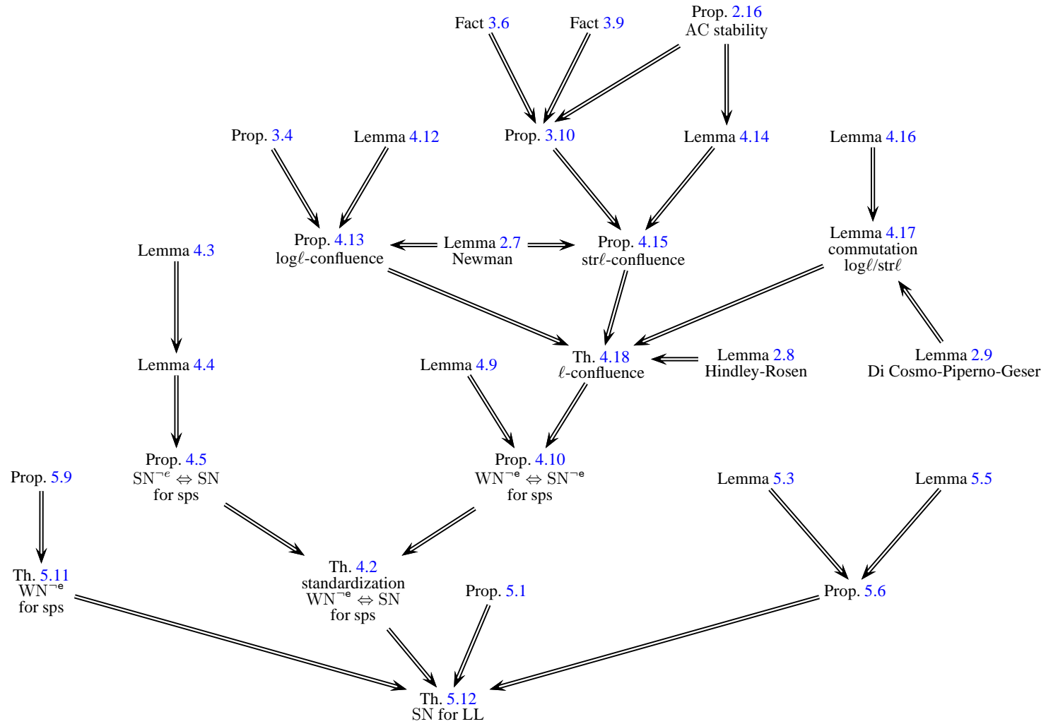
Figure 1. Dependencies between the results of this paper.
