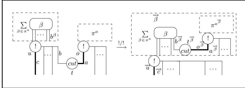
Figure 16: The (!/!) case of the proof of Proposition 3.10
