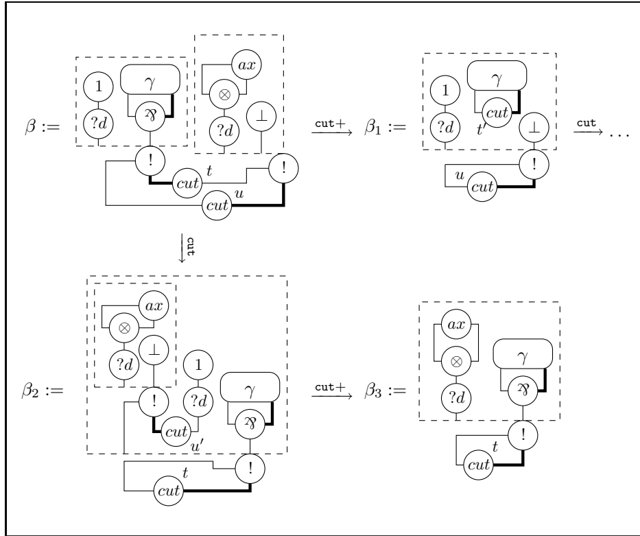
Figure 12: A counter-example to normalization and confluence of cut-elimination. The slice \gamma is obtained by removing the cut from the slice \alpha pictured in Figure 11
