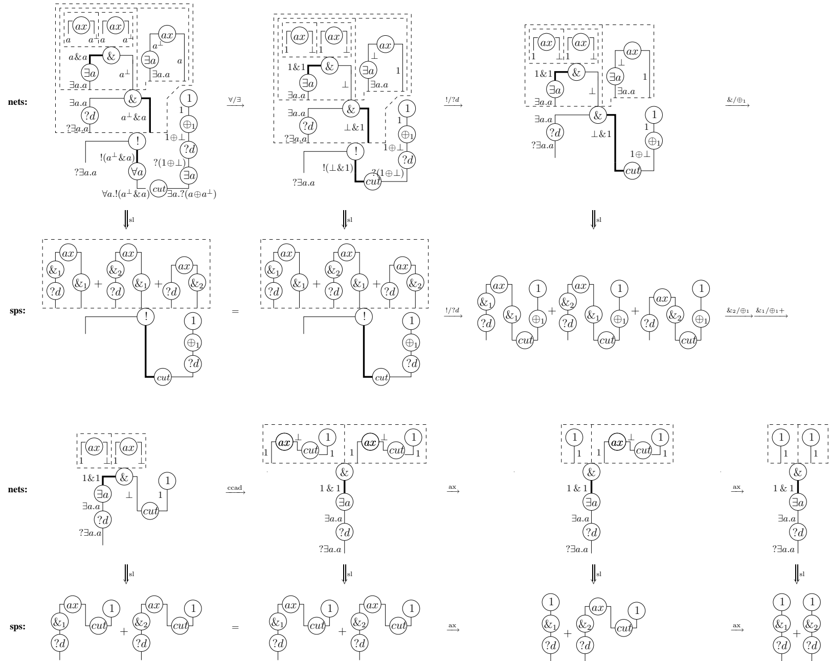
Figure 22. Example of how sps cut-elimination simulates that of nets: notice that the (ccad) and ( \forall/\exists ) steps are invisible in sps reduction
