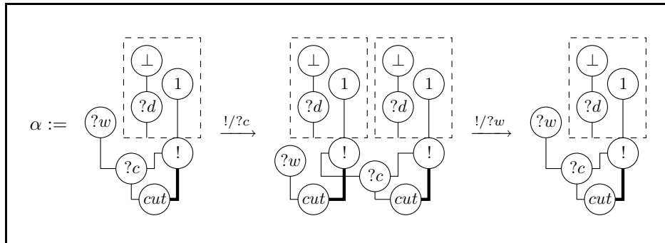
Figure 11: An example of slice \alpha s.t. \alpha \xrightarrow{cut+} \alpha . The slice \alpha is typable by LL formulas
