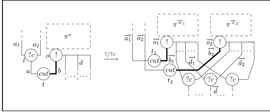
Figure 15: The (!/?c) case of the proof of Proposition 3.10
