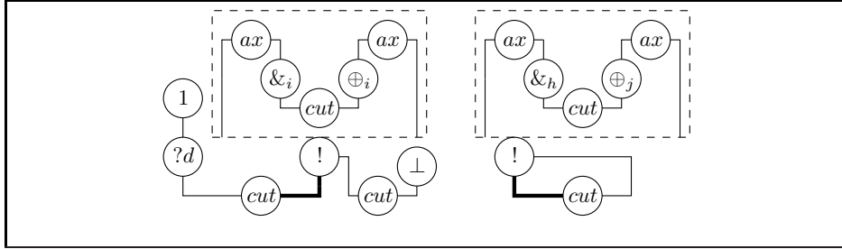
Figure 13: The multiset \text{sgth}(\pi) , where \pi is the sps of Fig. 3, consists of four single-threaded slices, given by the above picture taking i, h, j \in \{1, 2\} , h \neq j .
