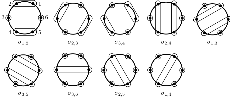
Figure 2: Generators of the dual monoid of type B for n = 3
