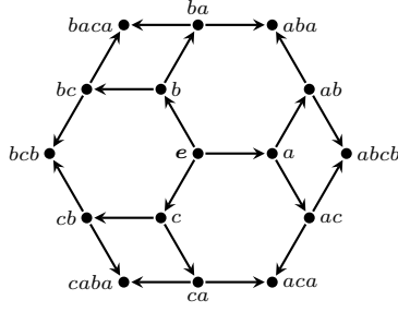
Figure 1: Hasse diagram of (\mathcal{S}, \leq_1) for the Artin-Tits monoid \mathbf{A} = \langle a, b, c \mid aba = bab, bcb = cbc, cac = aca \rangle . In this example, \mathcal{S} is not closed by left divisibility since, for instance, caba \in \mathcal{S} whereas cab \notin \mathcal{S} .
